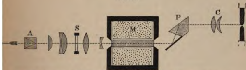
Projection of magnetic rotation of light. C, condensing lenses; P, reflecting polariser; magnetising coil surrounding bar of heavy glass; S, mica star of twenty-four rays; A, analyser (Ahrens's triple prism).
